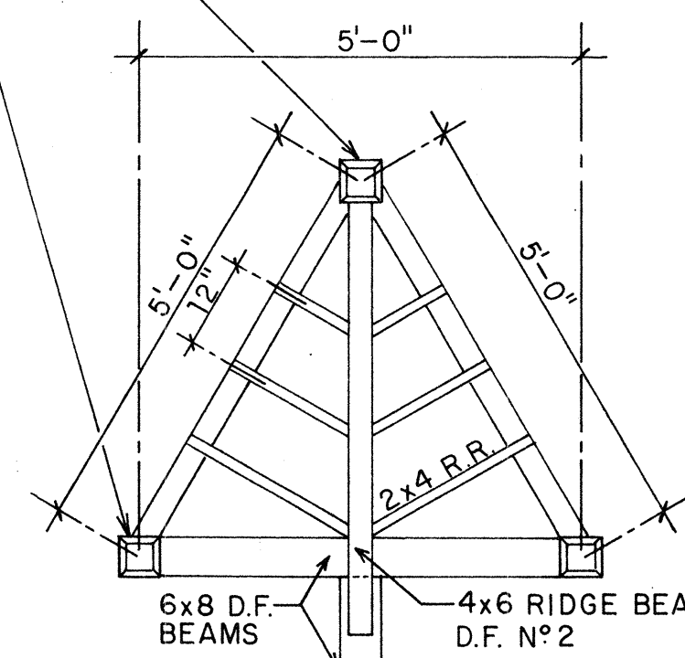
"ROOF" FRAMING
